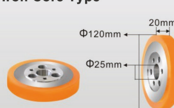
铁芯款 U0211 Iron Core Type
