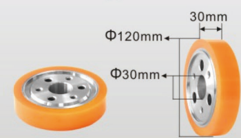
铁芯款 U0208 Iron Core Type
