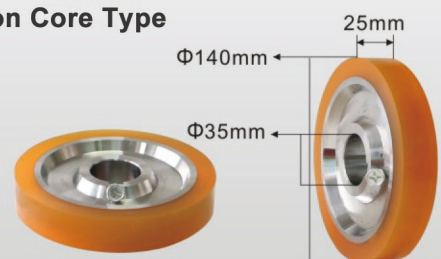
铁芯款 U0105 Iron Core Type
