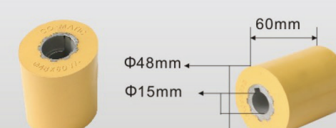
贝特原装款 U0401 Co-matic Original Type
