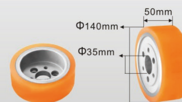
铁芯款 U0201 Iron Core Type
