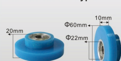
硅胶轮 U0518 Silicone Wheels Type
