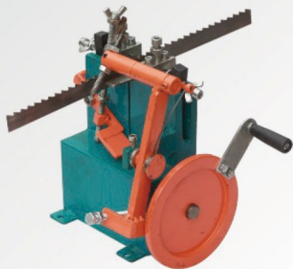
拼框门专用收紧器(第二代) Special tightening device for splicing frame door
