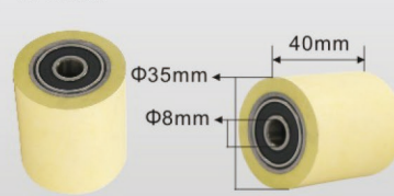
手动封边机轮 U0610 Manual Edge Bander Wheel
