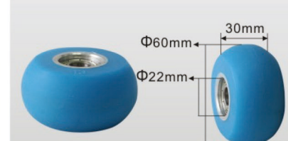
硅胶轮 U0511 Silicone Wheels Type
