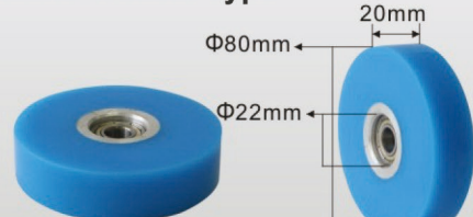
硅胶轮 U0508 Silicone Wheels Type
