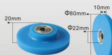
硅胶轮 U0510 Silicone Wheels Type
