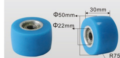
硅胶轮 U0514 Silicone Wheels Type
