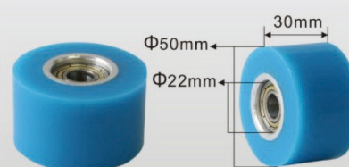
硅胶轮 U0509 Silicone Wheels Type
