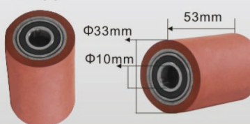
手动封边机轮 U0607 Manual Edge Bander Wheel
