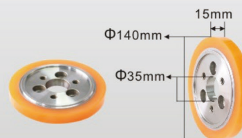
铁芯款 U0205 Iron Core Type
