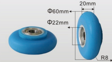
硅胶轮 U0516 Silicone Wheels Type
