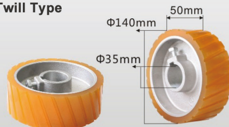
斜纹款 U0101X Twill Type
