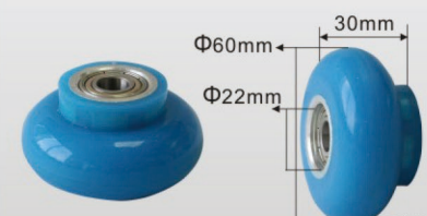
硅胶轮 U0512 Silicone Wheels Type
