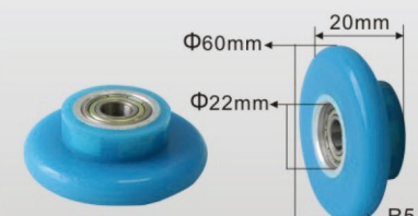
硅胶轮 U0513 Silicone Wheels Type
