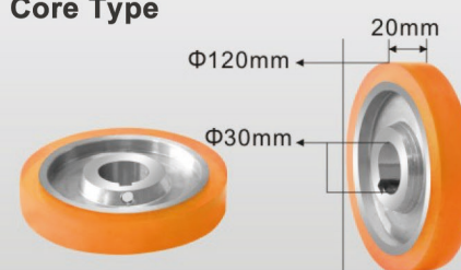
铁芯款 U0107 Iron Core Type
