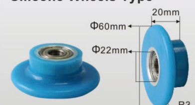
硅胶轮 U0515 Silicone Wheels Type
